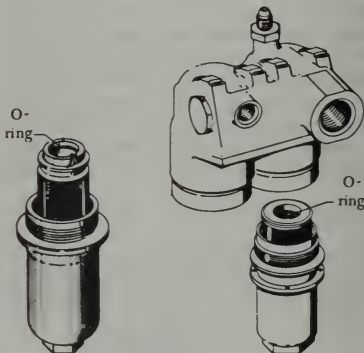
FIGURE 6-27. Filtering assembly.
